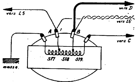
Branchement 123 V.
