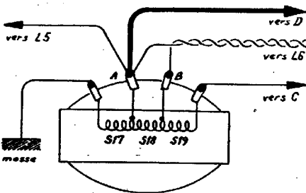
Branchement 117 V.
